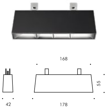
CEILING 4 LED plug-in comfort Downlight lineare fisso IP65
