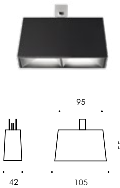
CEILING 2 LED plug-in comfort Downlight lineare fisso IP65
