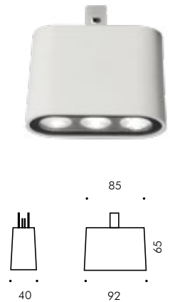
TRENDY 3 LED plug-in Downlight fisso IP65
